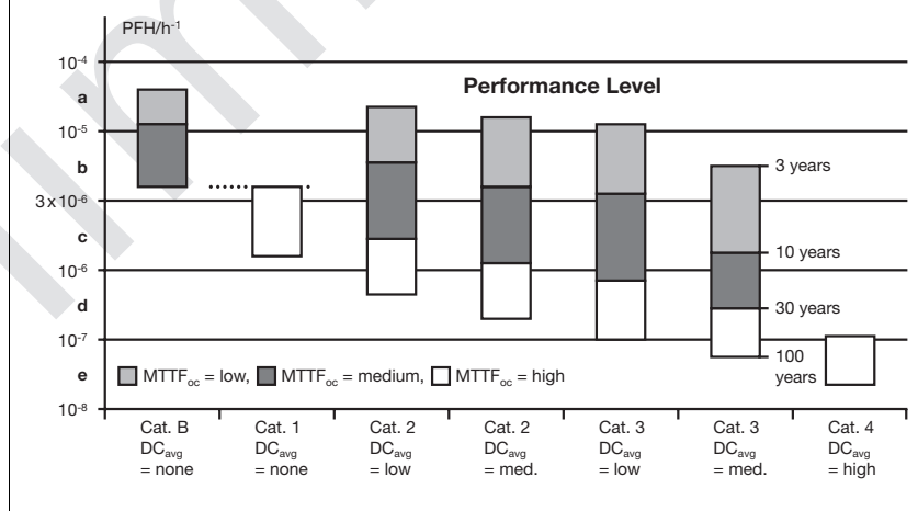
Relationship between categories DC, MTTF_D and PL
